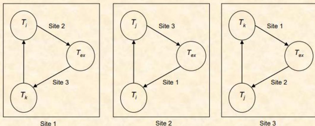
Fig. Distributed Deadlock Detection
